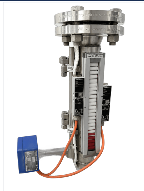
Fig.: Level control
